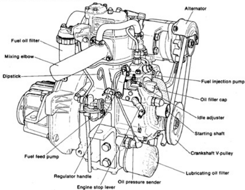
1-1.2 Exhaust side viewed from bow / starboard
