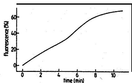
FIGURE 7: Spontaneous collapse of an imposed transbilayer \Delta\text{pH} during continued slow fusion of CL/DOPC/Chol vesicles containing oleic acid. \text{Ca}^{2+} concentration was 10 mM. Note the difference in time scale relative to that in Figures 1, 3, 5, and 6.
