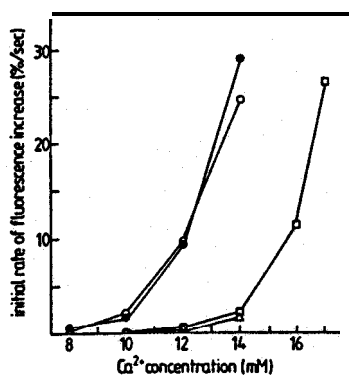
FIGURE 4: Effect of a transbilayer pH gradient on the initial rate of the \text{Ca}^{2+} -induced fusion of CL/DOPC/Chol vesicles with or without oleic acid. Triangles, vesicles with 20 mol% OA in the presence of a \Delta\text{pH} (rates after the points of inflection, see Figure 3A); squares, vesicles without OA in the presence of a \Delta\text{pH} ; open circles, OA-containing vesicles, pretreated with nigericin/valinomycin, in the presence of an imposed \Delta\text{pH} (the rate of fusion was determined from the steepest part of the curve, see Figure 5); closed circles, OA-containing vesicles at pH 7.5 in the absence of a \Delta\text{pH} .
