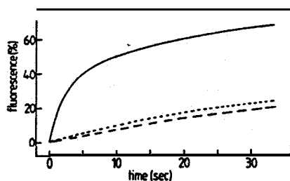
FIGURE 1: Effect of oleic acid on the \text{Ca}^{2+} -induced fusion of CL/DOPC/Chol (1:1:1) vesicles. \text{CaCl}_2 concentration was 12 mM. Drawn line, vesicles containing 20 mol% OA at pH 7.5 in the absence of a \Delta\text{pH} ; dotted line, vesicles containing 20 mol% OA at pH 6.0 in the absence of a \Delta\text{pH} (in this case, the standard 10 mM HEPES inside the vesicles and in the fusion medium was replaced by 10 mM MES, adjusted to pH 6.0); dashed line, vesicles without OA at pH 7.5 in the absence of a \Delta\text{pH} .
